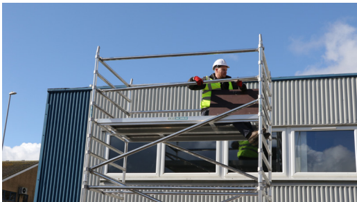
17. From a seated position using the 3T method, fit 4 horizontal braces above the appropriate rungs.
