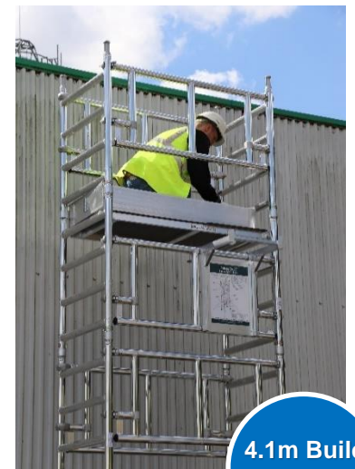
30. Fit toeboard.
