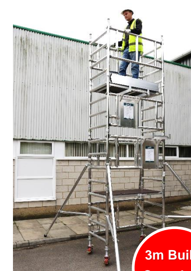
30. Access the platform using the trapdoor and unfold the toeboard.
