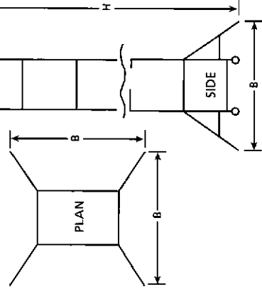
Fig. 4 TOWER WITH STABILISERS
